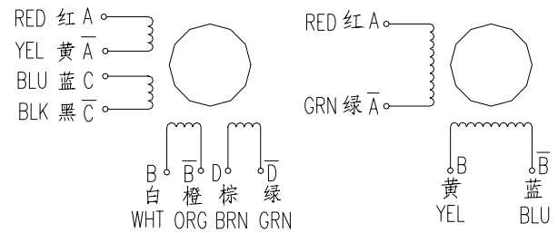
UNI/BI-POLAR(8 LEADS)
