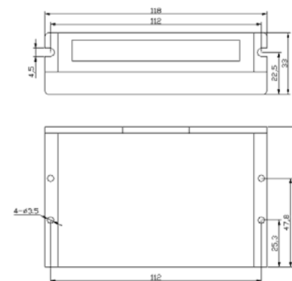
Figure 1: Mechanical specifications
