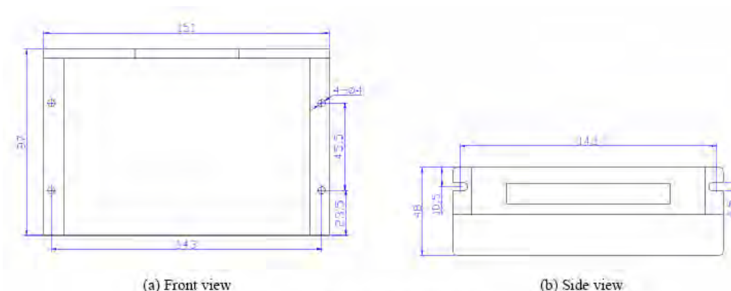
Figure 1: Mechanical specifications
