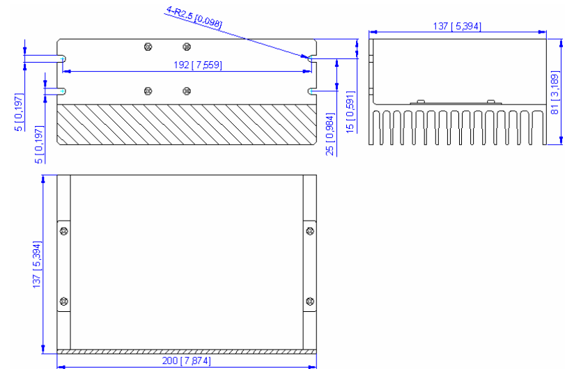
Figure 1: Mechanical specifications
